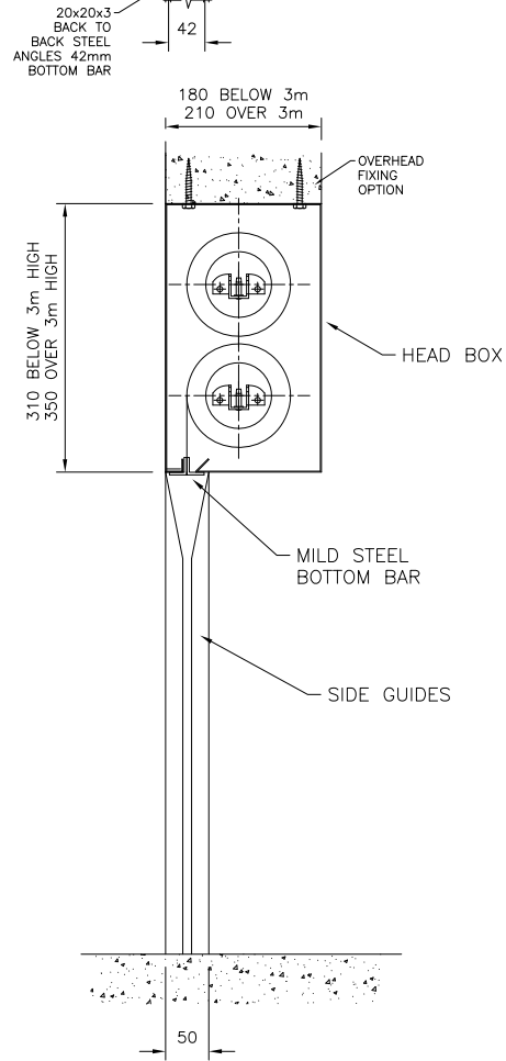
SECTION THROUGH HEAD BOX
