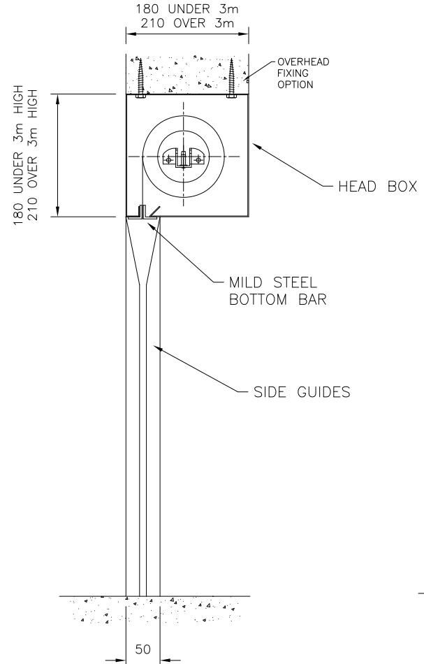
SECTION THROUGH HEAD BOX
