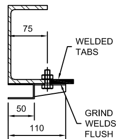
TYPICAL STEEL STRUCTURE (BY OTHERS)
